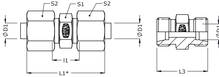
2D Assembly
