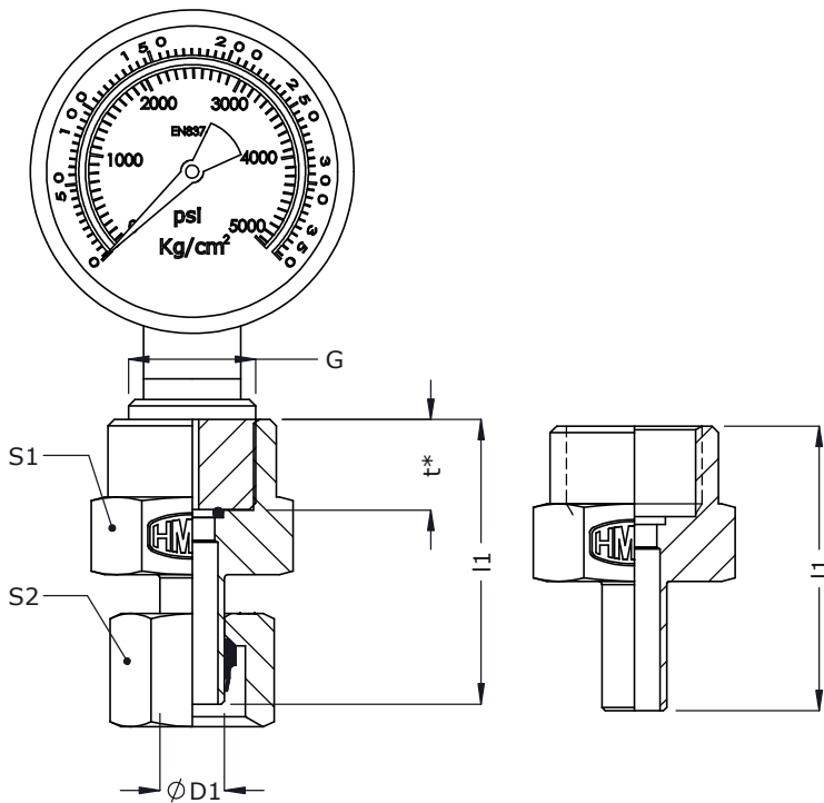
2D Assembly
