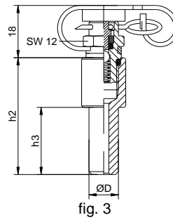
type BE test coupling for compression ring fittings
