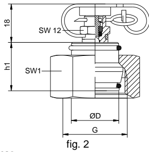
type DKO test coupling with 24° taper adaptor
