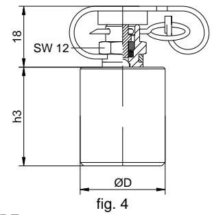
type BE test coupling for compression ring fittings
