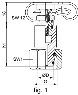
type DKO test coupling with 24° taper adaptor
